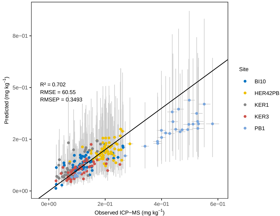
Sr PLS_kfold – ACE Predicted vs Observed (with errors)
