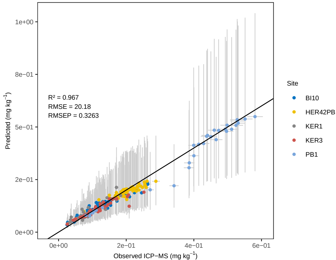
Sr RF – ACE Predicted vs Observed (with errors)
