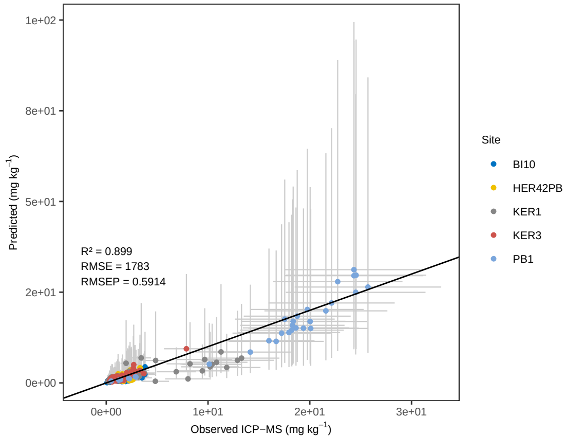
Ti Bayes – ACE Predicted vs Observed (with errors)
