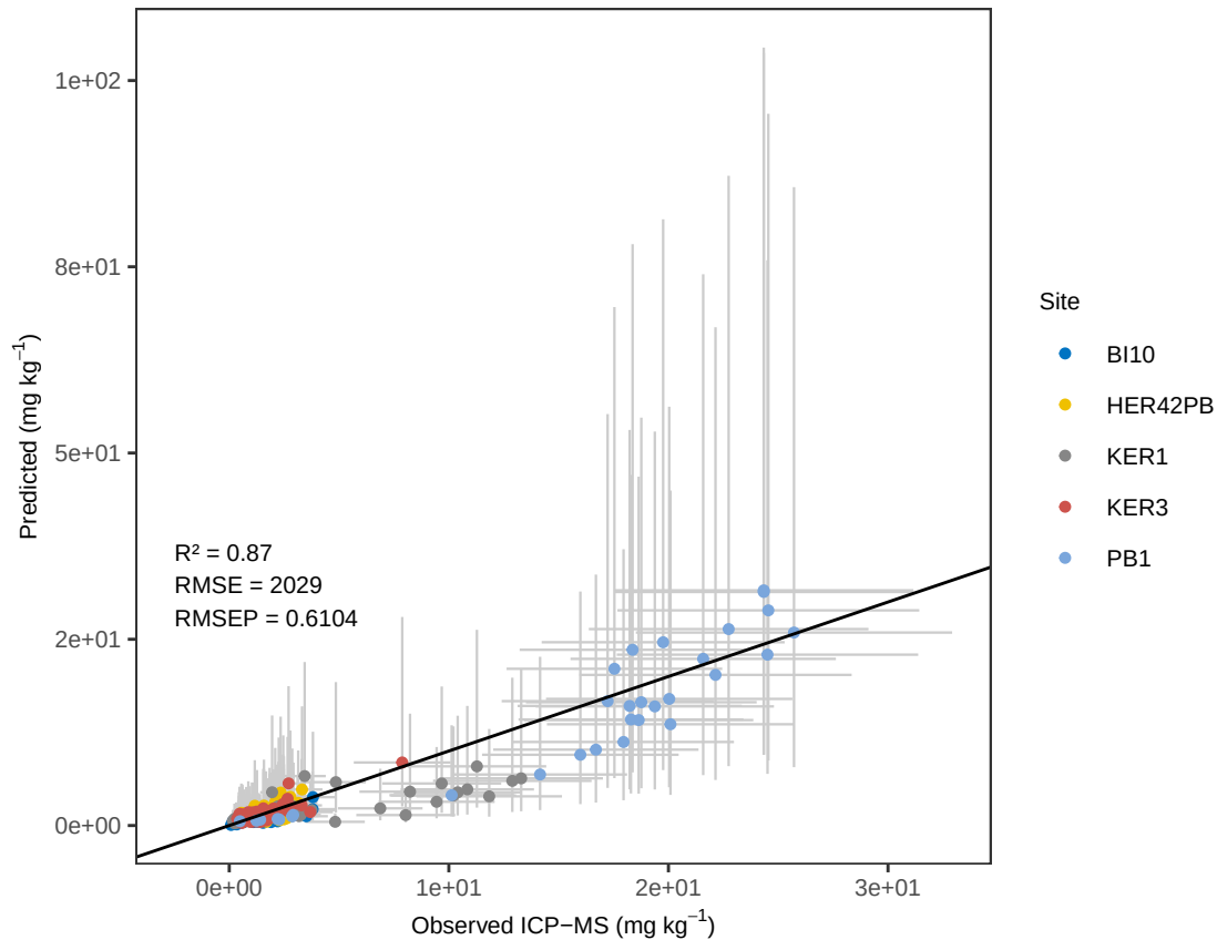
Ti PLS_LOO – ACE Predicted vs Observed (with errors)
