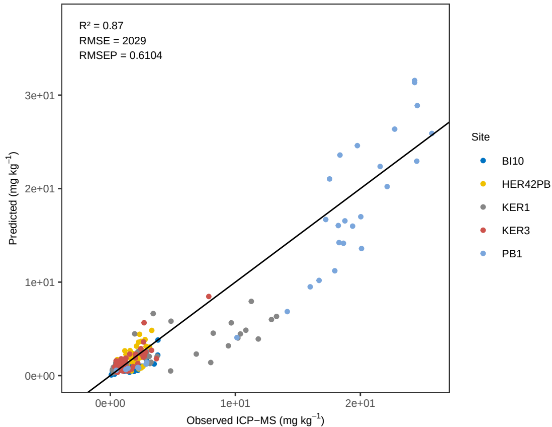
Ti PLS_kfold – ACE Predicted vs Observed
