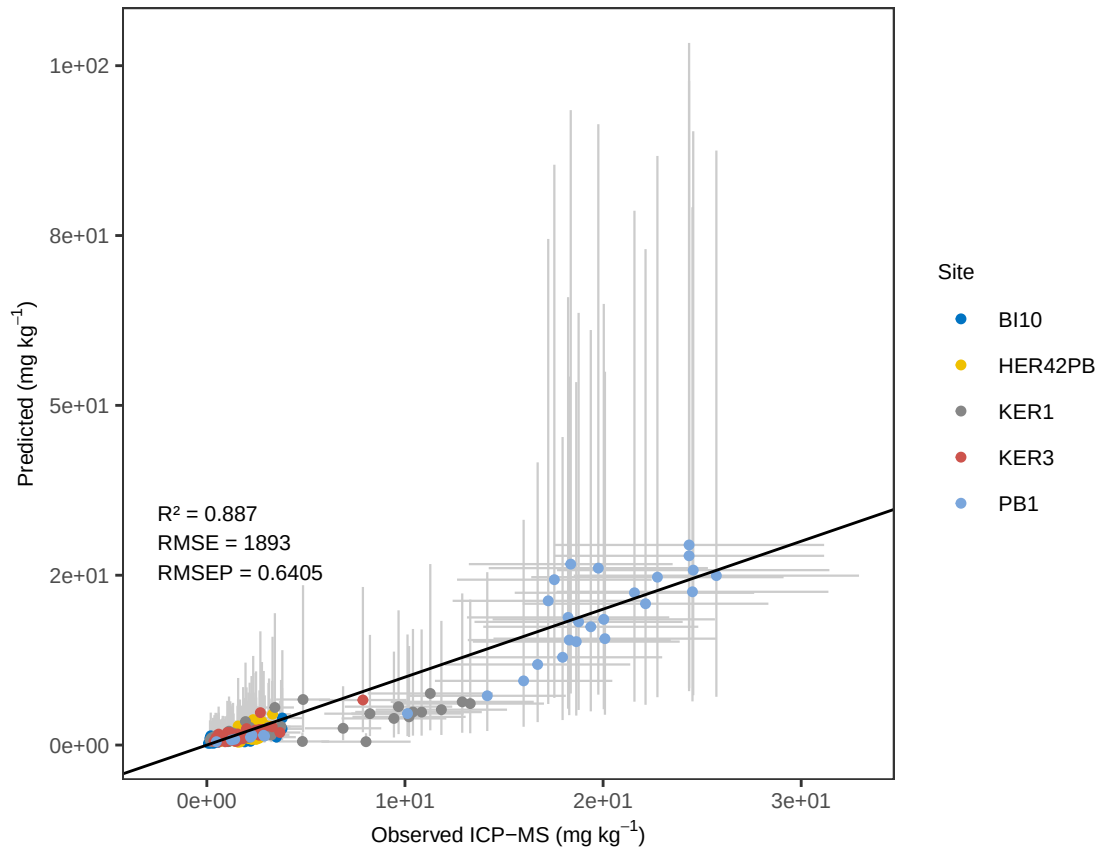
Ti WLS_weighted – ACE Predicted vs Observed (with errors)
