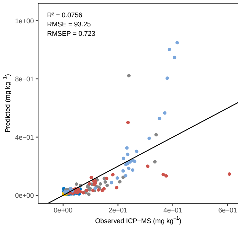
Zr PLS_LOO – ACE Predicted vs Observed
