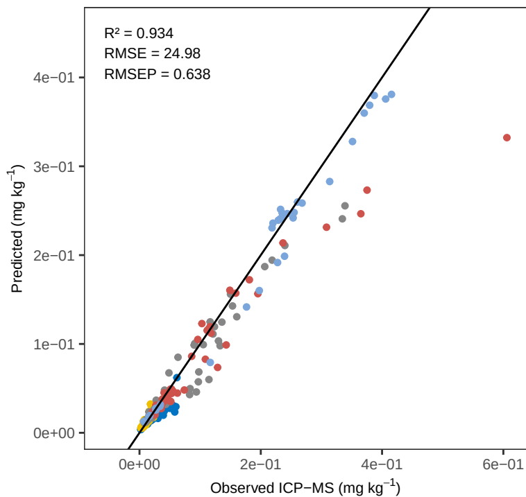
Zr RF – ACE Predicted vs Observed
