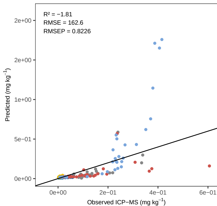
Zr WLS_weighted – ACE Predicted vs Observed
