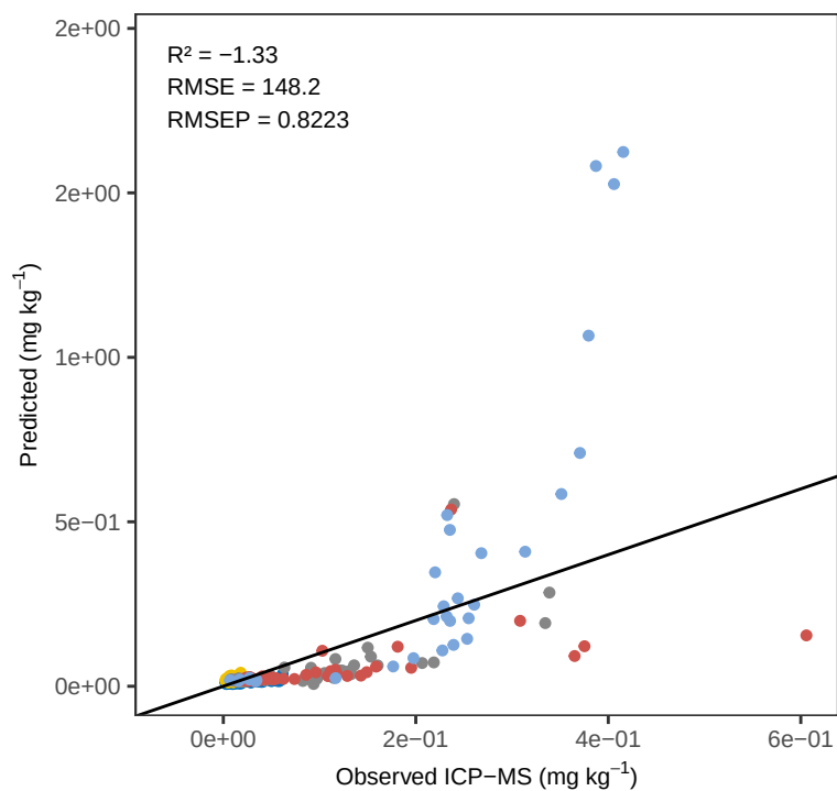
Zr OLS – ACE Predicted vs Observed
