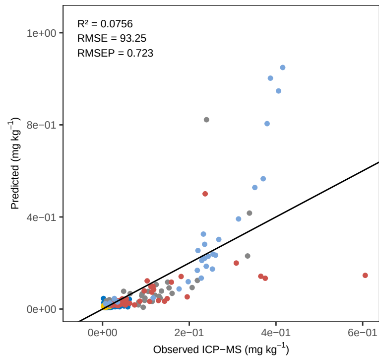
Zr PLS_kfold – ACE Predicted vs Observed
