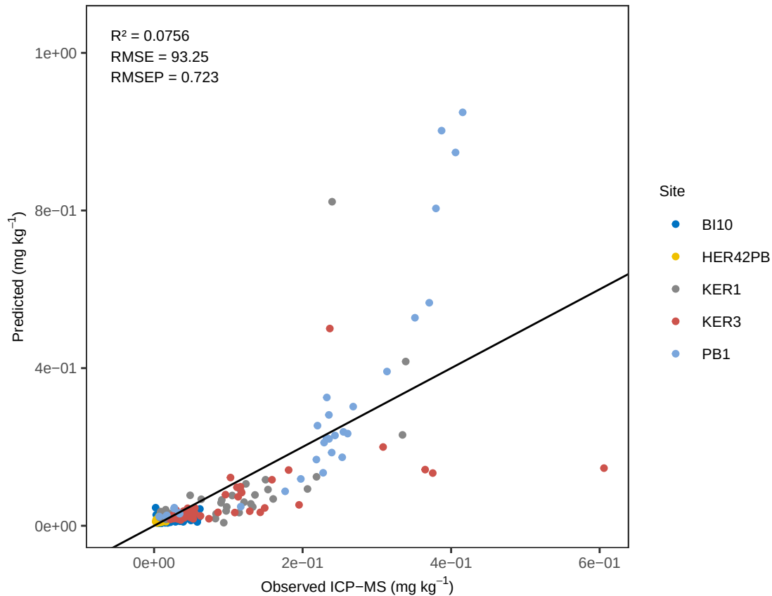
Zr PLS_LOO – ACE Predicted vs Observed
