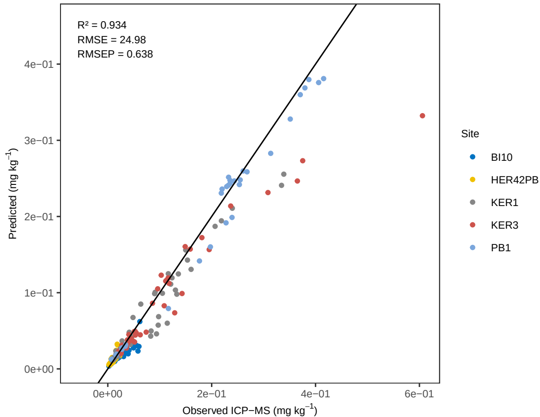
Zr RF – ACE Predicted vs Observed
