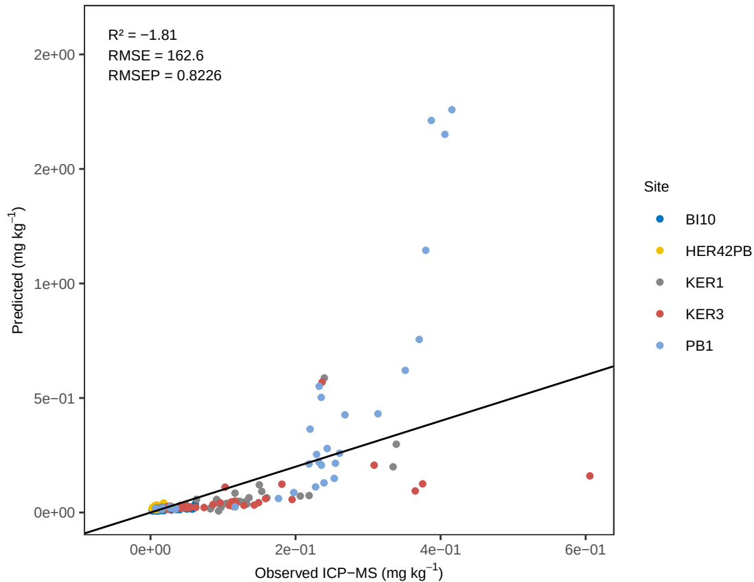
Zr WLS_weighted – ACE Predicted vs Observed
