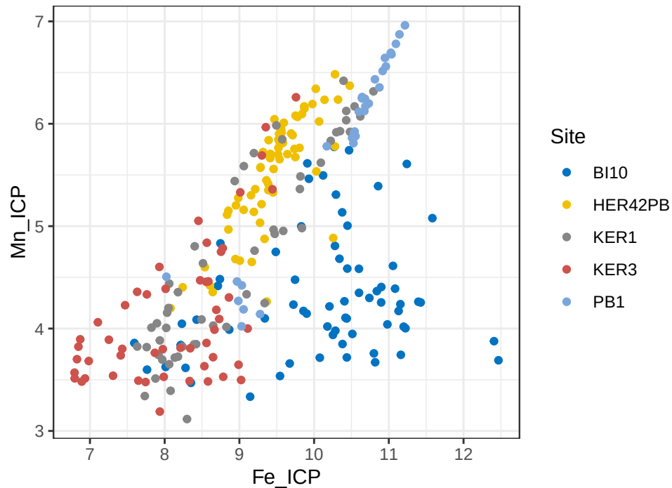
ICP relationship: Fe_ICP vs Mn_ICP
