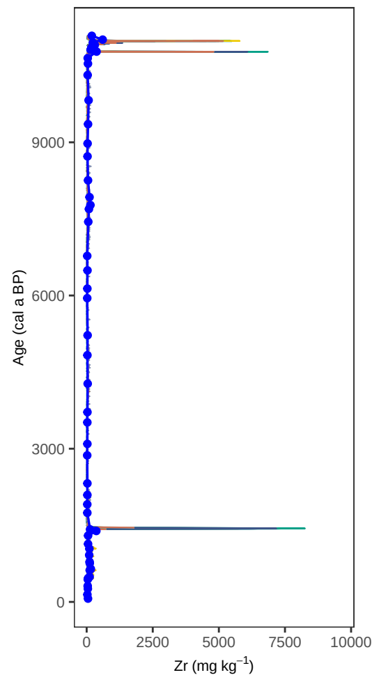
Site KER3 – Zr (age, all models)
