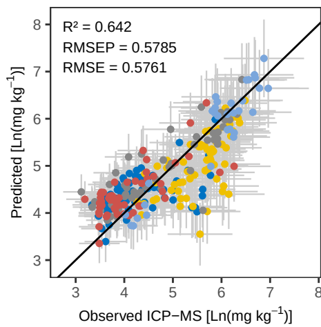
Mn WLS – Predicted vs Observed
