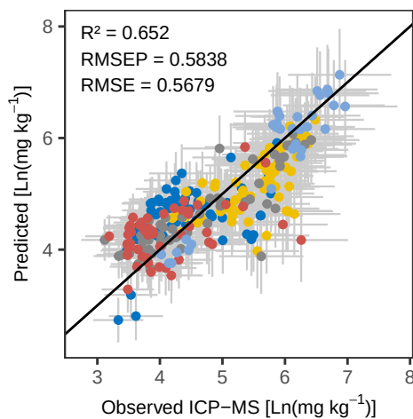
Mn PLS_kfold – Predicted vs Observed
