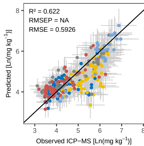
Mn WLS_weighted – Predicted vs Observed
