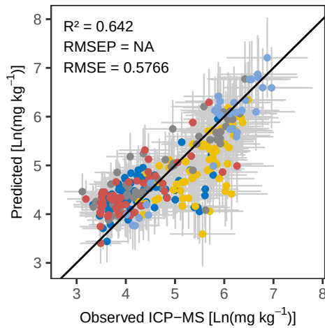
Mn Bayes – Predicted vs Observed
