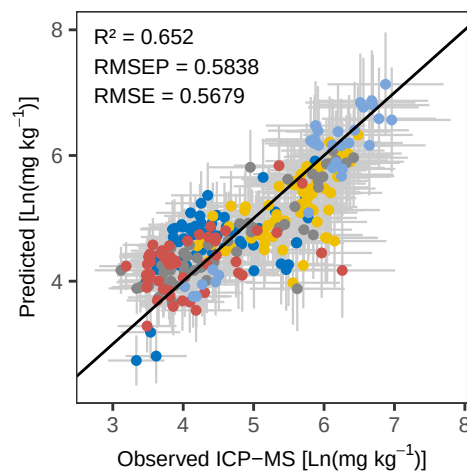
Mn PLS_LOO – Predicted vs Observed
