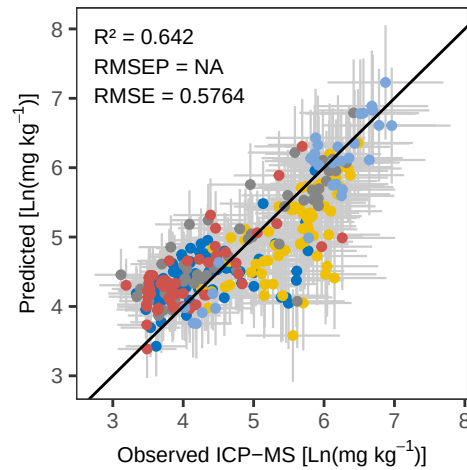
Mn RF – Predicted vs Observed
