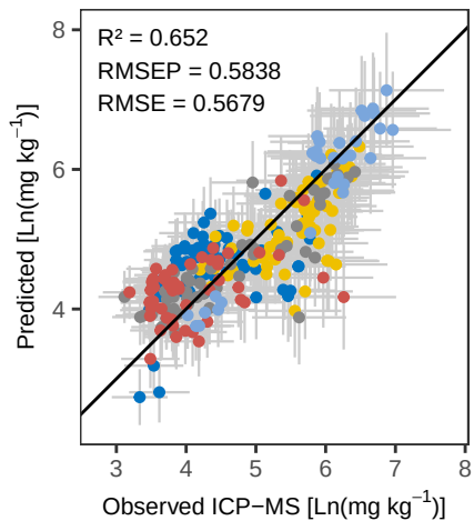
Mn PLS_LOO – Predicted vs Observed
