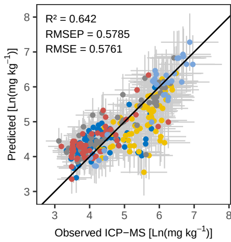
Mn WLS – Predicted vs Observed
