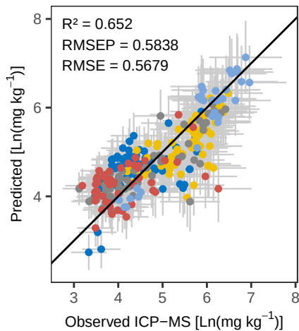
Mn PLS_kfold – Predicted vs Observed
