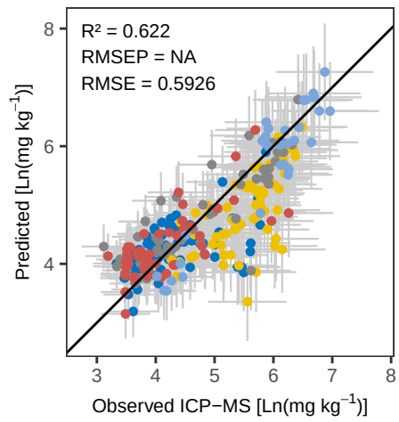
Mn WLS_weighted – Predicted vs Observed
