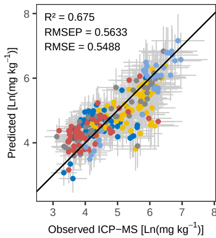
Mn PLS_kfold – Predicted vs Observed
