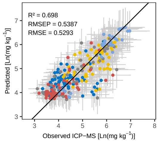
Mn PLS_LOO – Predicted vs Observed
