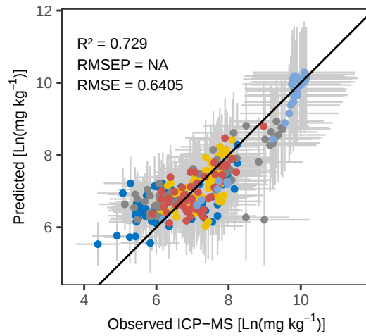
Ti RF – Predicted vs Observed
