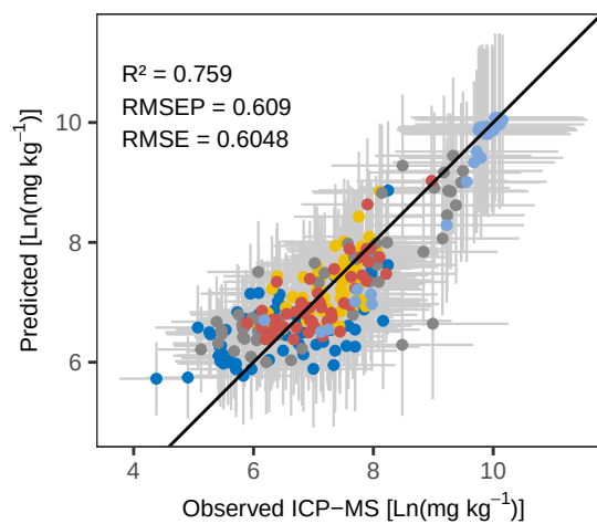
Ti PLS_LOO – Predicted vs Observed
