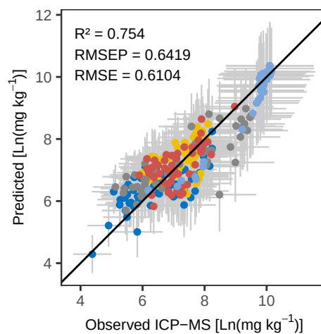
Ti PLS_LOO – Predicted vs Observed
