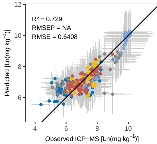
Ti Bayes – Predicted vs Observed
