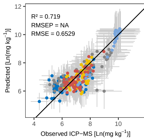
Ti WLS_weighted – Predicted vs Observed
