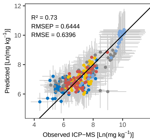
Ti WLS – Predicted vs Observed
