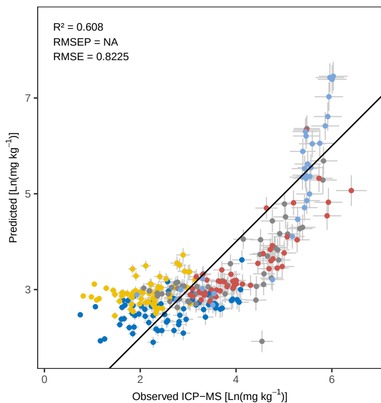
Zr WLS – Predicted vs Observed
