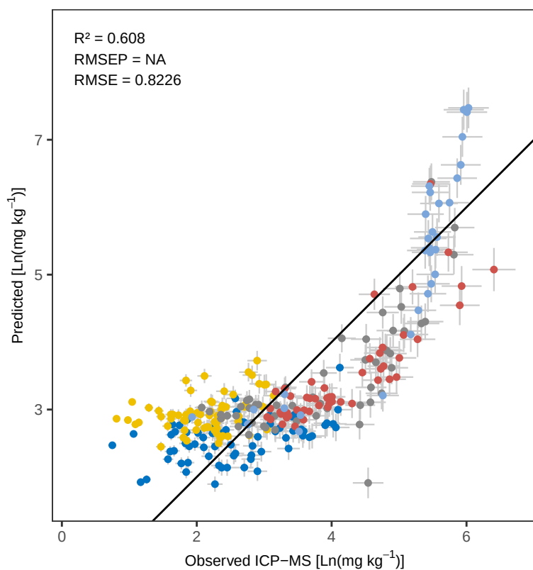
Zr WLS_weighted – Predicted vs Observed
