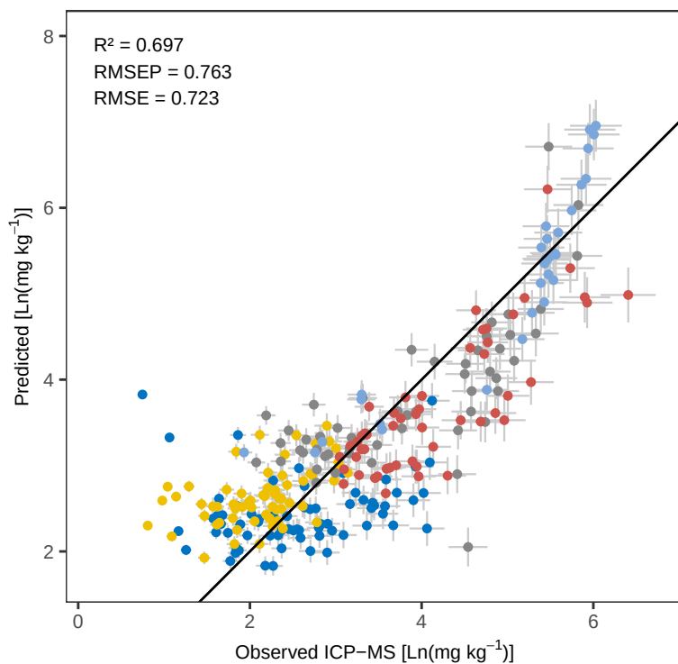
Zr PLS_LOO – Predicted vs Observed
