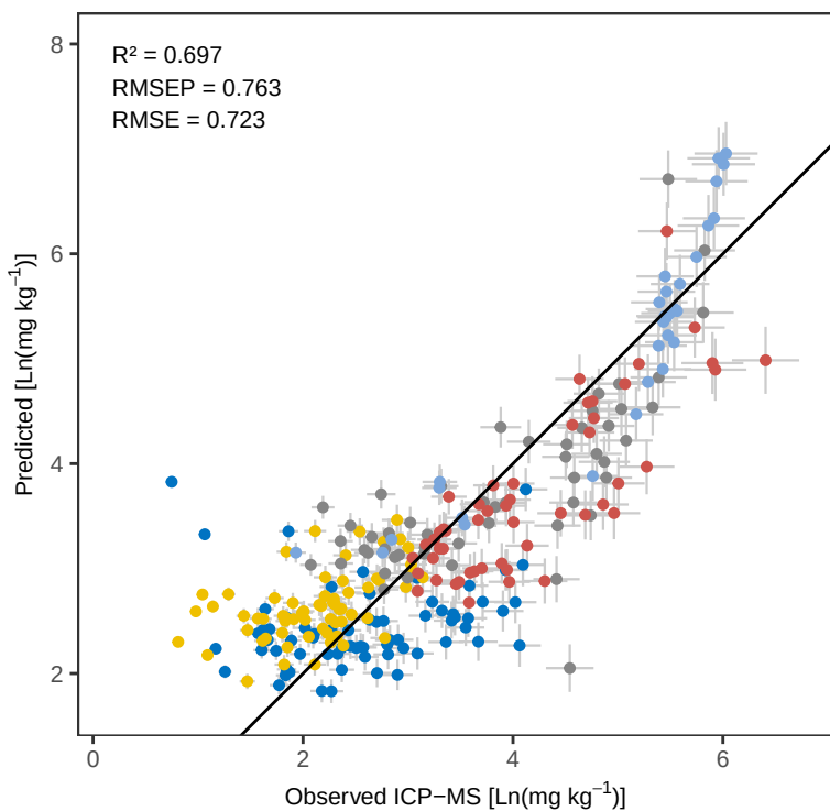
Zr PLS_kfold – Predicted vs Observed
