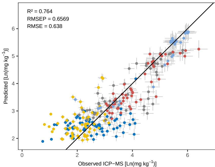
Zr RF – Predicted vs Observed
