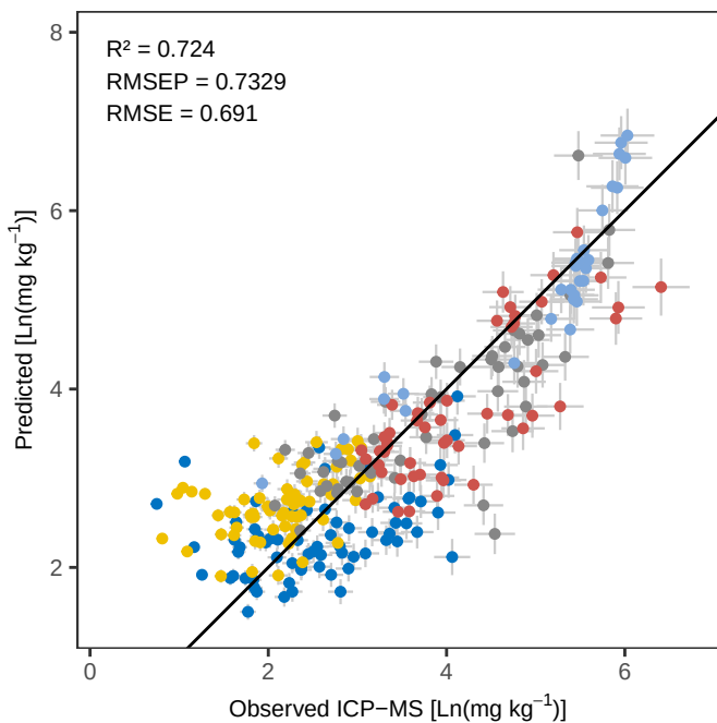
Zr Bayes – Predicted vs Observed
