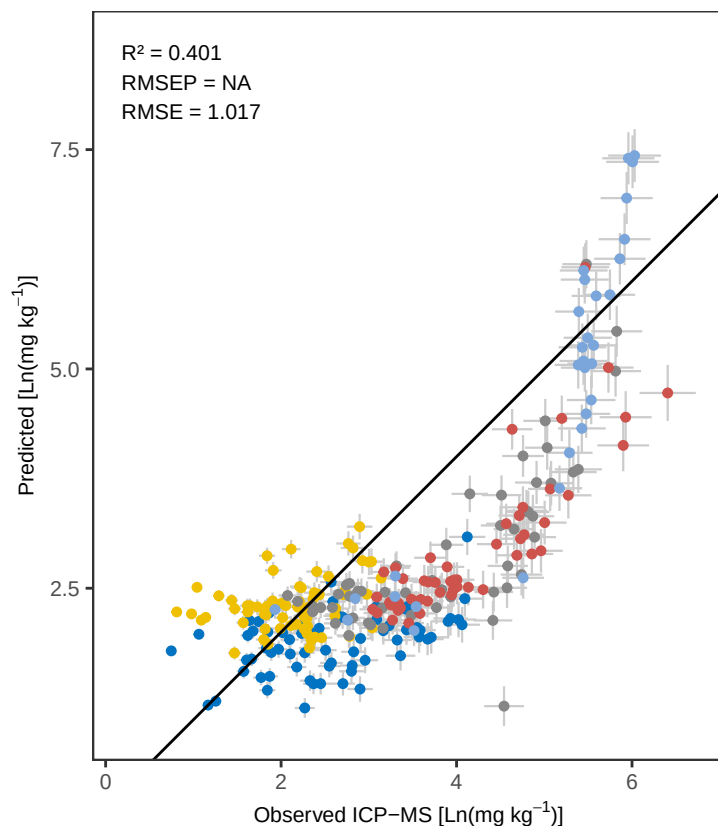
Zr OLS_weighted – Predicted vs Observed
