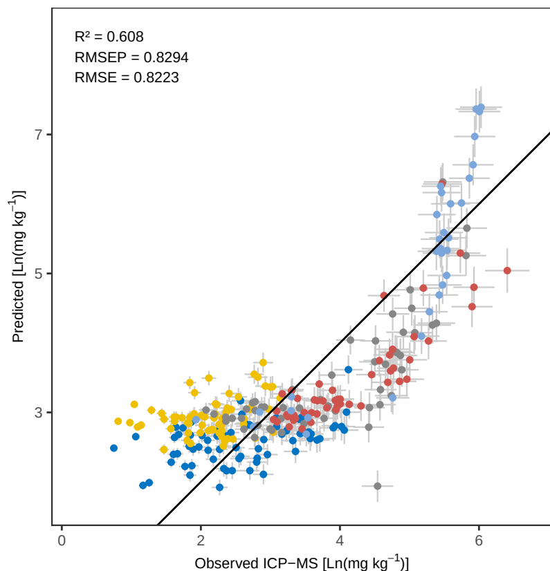
Zr OLS – Predicted vs Observed
