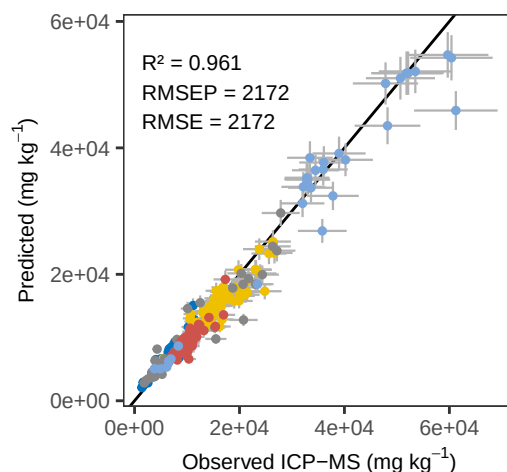
Ca PLS_LOO – ACE Predicted vs Observed
