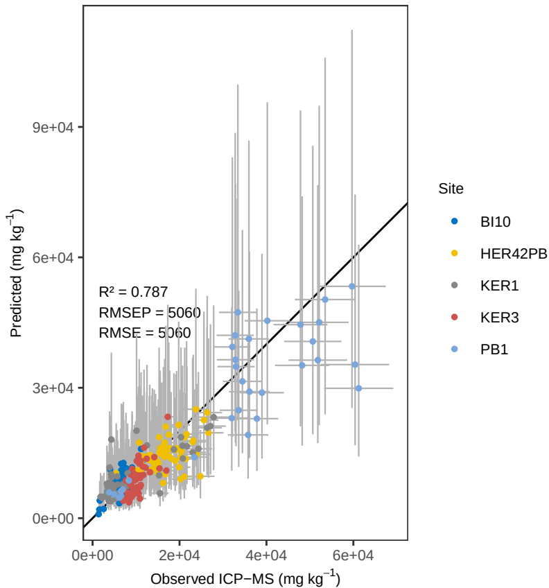
Ca PLS_LOO - ACE Predicted vs Observed
