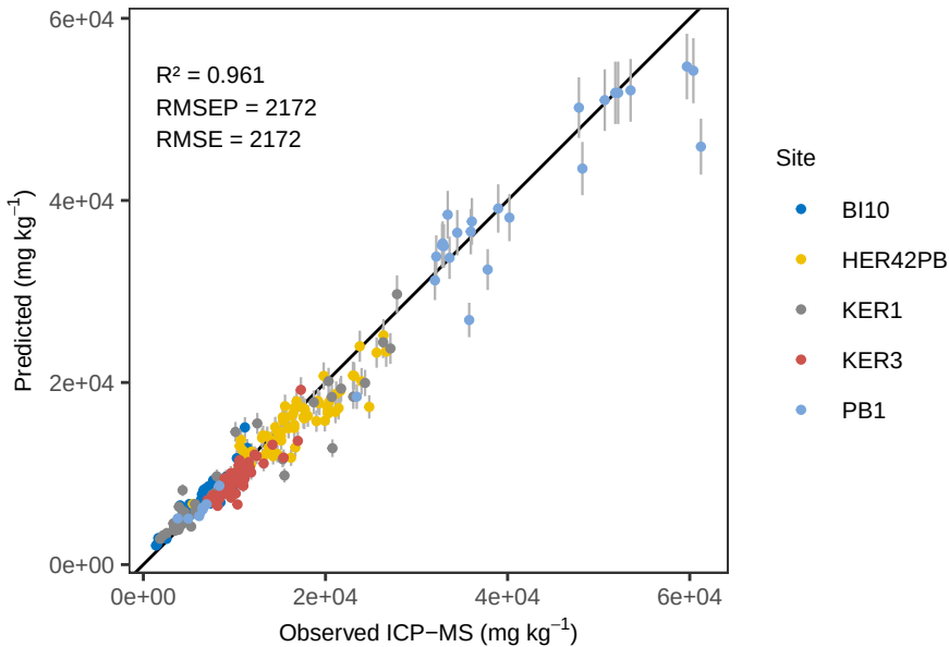
Ca RF – ACE Predicted vs Observed
