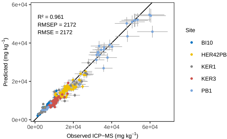
Ca RF – ACE Predicted vs Observed
