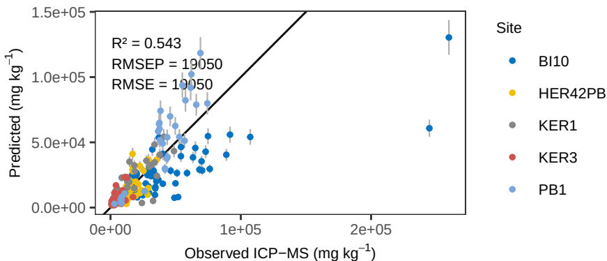
Fe OLS – ACE Predicted vs Observed
