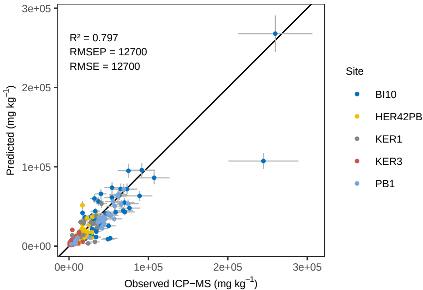
Fe PLS_LOO – ACE Predicted vs Observed
