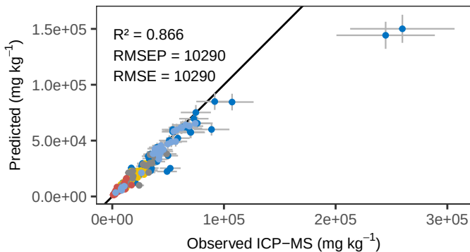
Fe RF – ACE Predicted vs Observed
