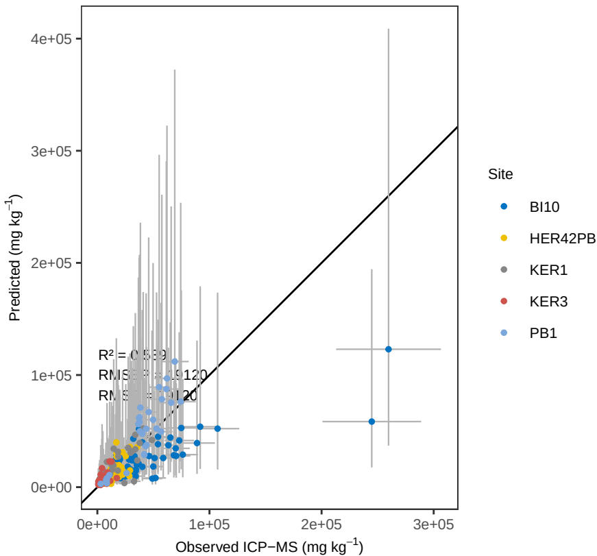
Fe WLS_weighted – ACE Predicted vs Observed
