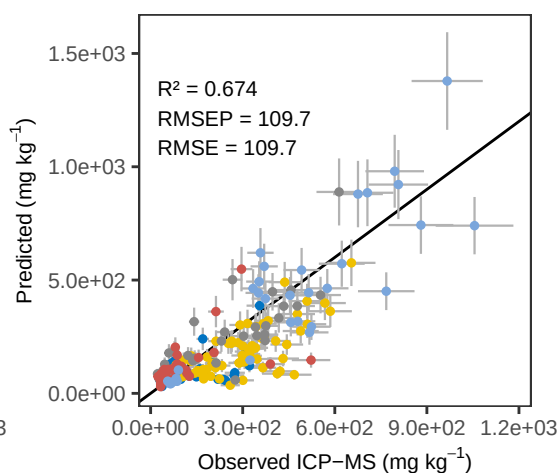
Mn RF – ACE Predicted vs Observed
