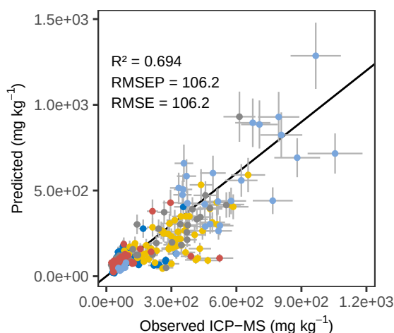
Mn PLS_kfold – ACE Predicted vs Observed
