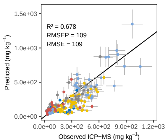
Mn Bayes – ACE Predicted vs Observed
