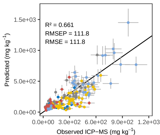
Mn WLS – ACE Predicted vs Observed
