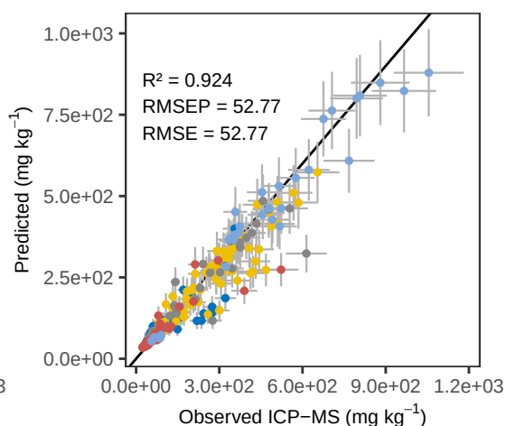
Mn PLS_LOO – ACE Predicted vs Observed
