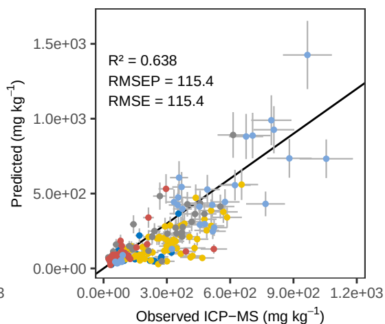
Mn WLS_weighted – ACE Predicted vs Observed
