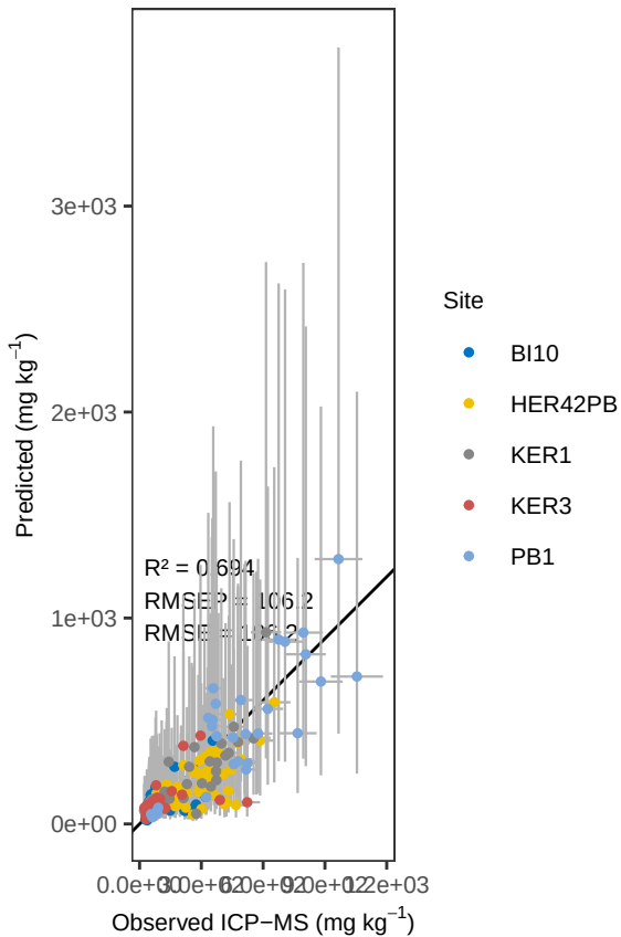
Mn Bayes – ACE Predicted vs Observed
