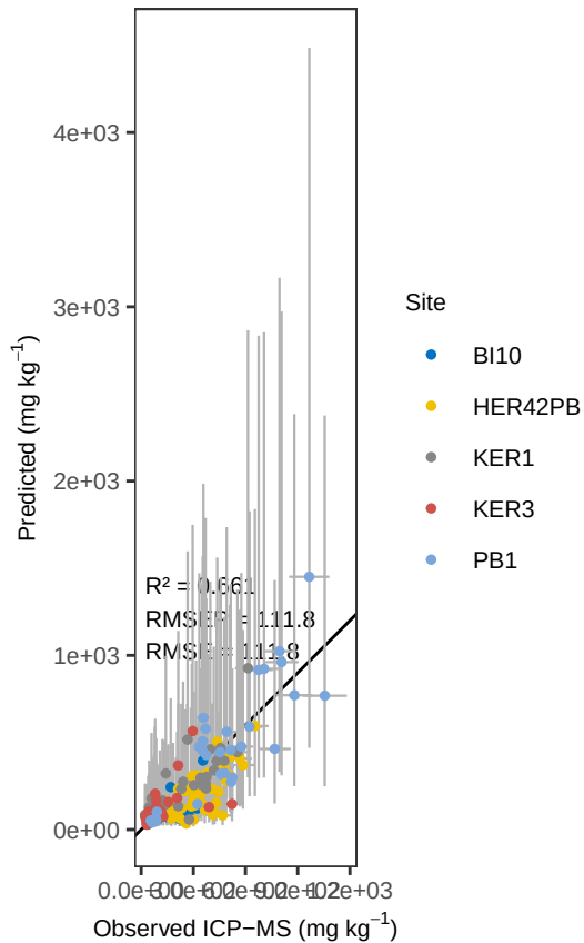
Mn OLS – ACE Predicted vs Observed
