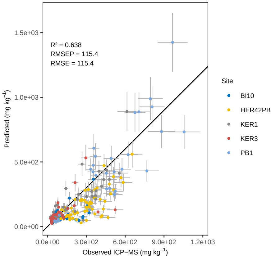
Mn OLS_weighted – ACE Predicted vs Observed
