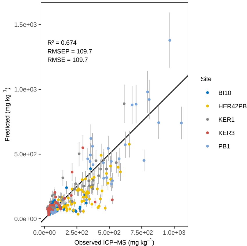
Mn WLS_weighted – ACE Predicted vs Observed
