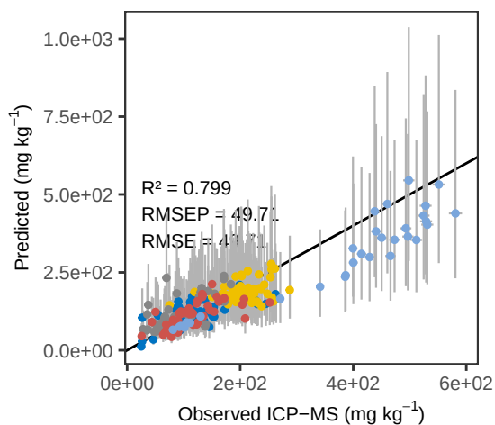
Sr PLS_kfold – ACE Predicted vs Observed
