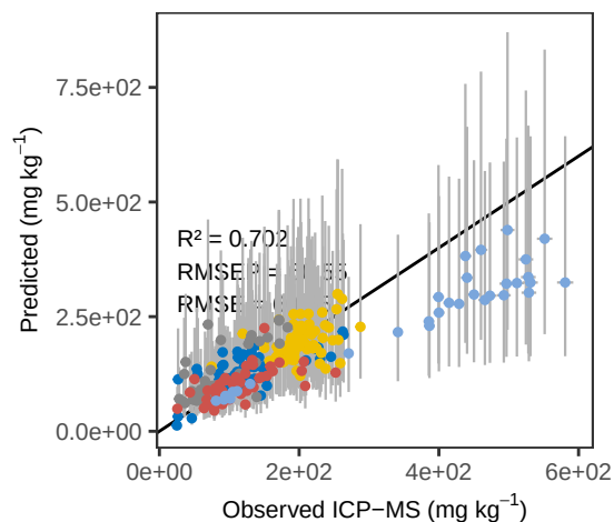
Sr PLS_LOO – ACE Predicted vs Observed
