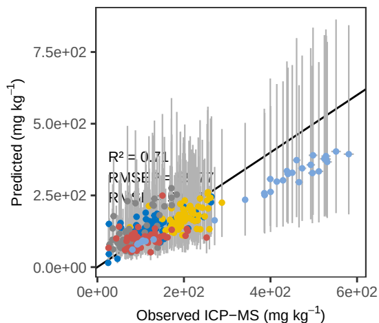
Sr WLS – ACE Predicted vs Observed
