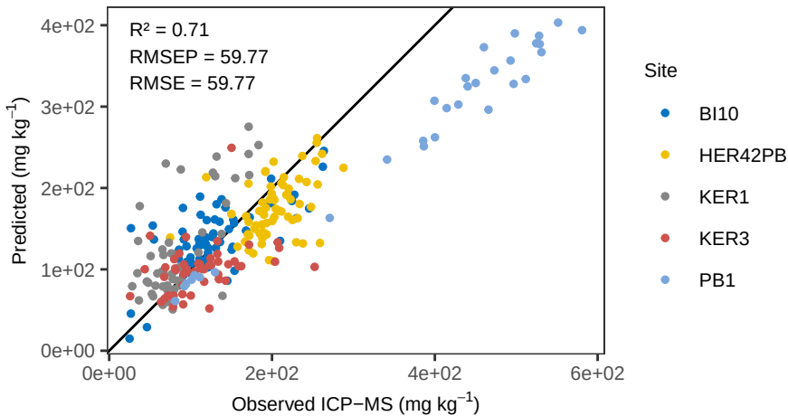
Sr OLS – ACE Predicted vs Observed
