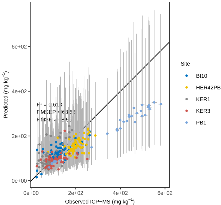
Sr OLS_weighted – ACE Predicted vs Observed
