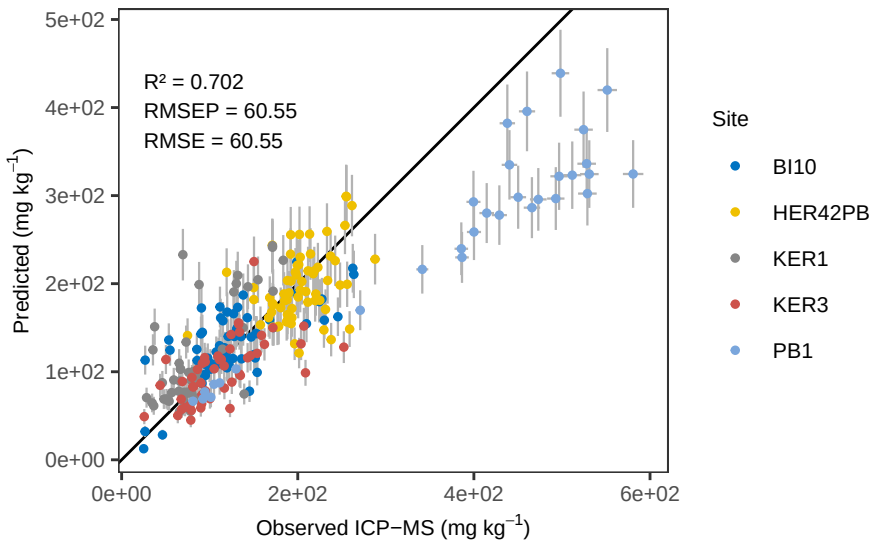
Sr PLS_LOO – ACE Predicted vs Observed
