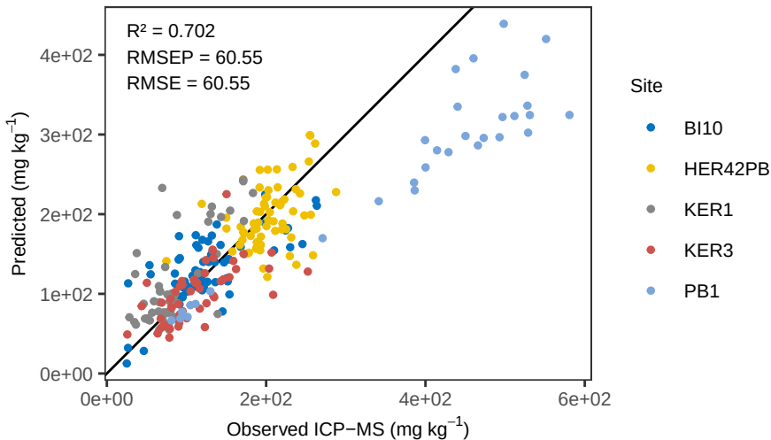
Sr PLS_kfold – ACE Predicted vs Observed
