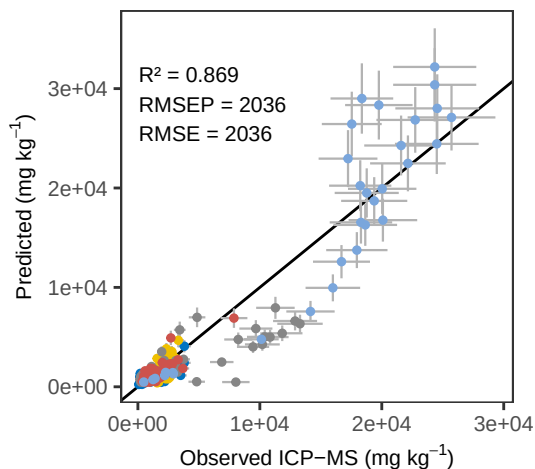
Ti WLS – ACE Predicted vs Observed
