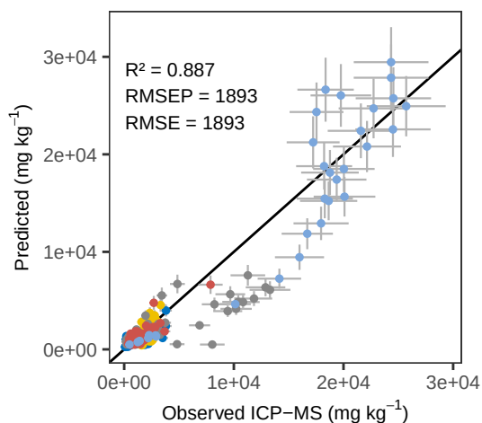
Ti RF – ACE Predicted vs Observed
