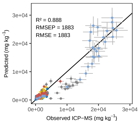
Ti Bayes – ACE Predicted vs Observed
