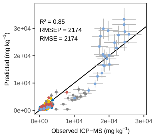
Ti WLS_weighted – ACE Predicted vs Observed
