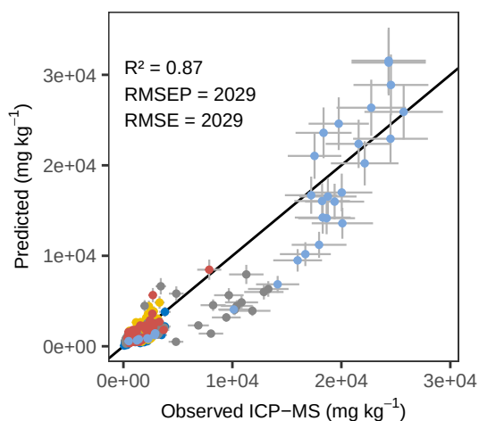
Ti PLS_LOO – ACE Predicted vs Observed
