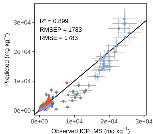
Ti PLS_kfold – ACE Predicted vs Observed
