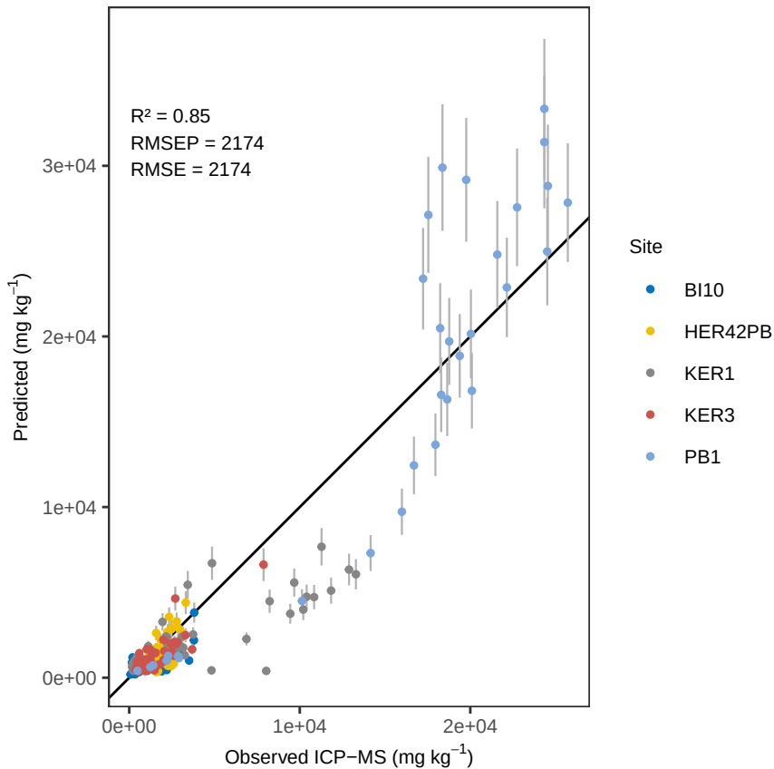
Ti OLS_weighted – ACE Predicted vs Observed
