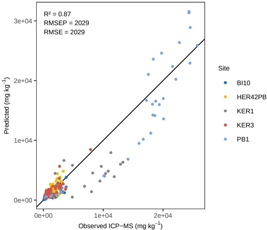
Ti PLS_LOO – ACE Predicted vs Observed
