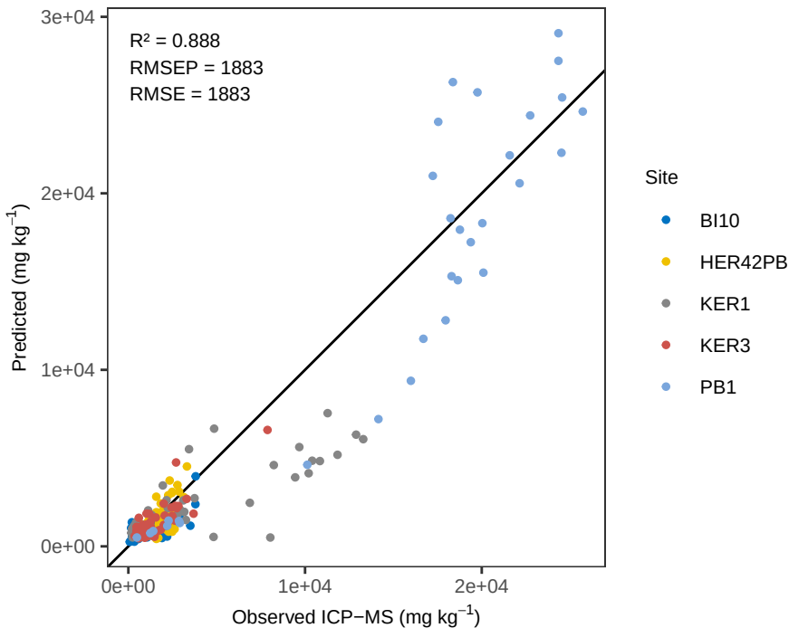
Ti WLS – ACE Predicted vs Observed
