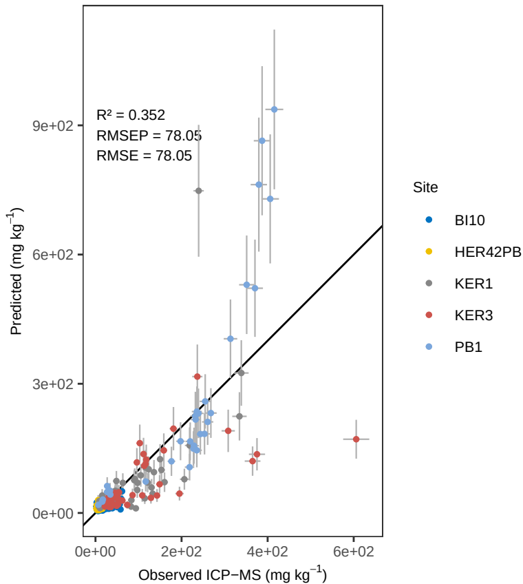
Zr Bayes – ACE Predicted vs Observed
