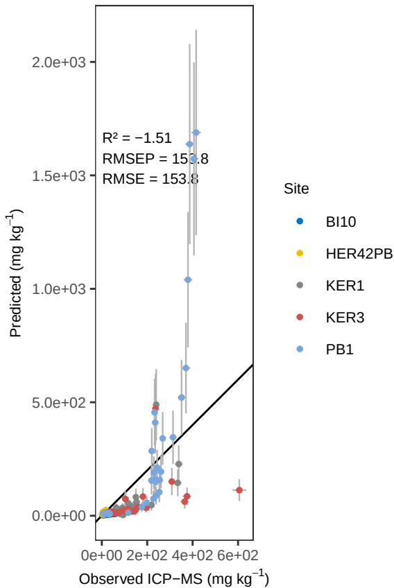
Zr OLS_weighted - ACE Predicted vs Observed
