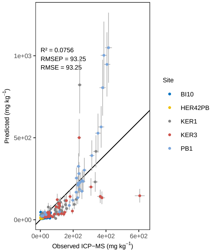
Zr PLS_LOO – ACE Predicted vs Observed
