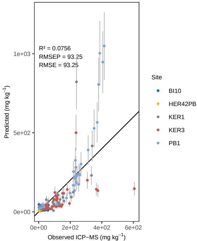
Zr PLS_kfold – ACE Predicted vs Observed
