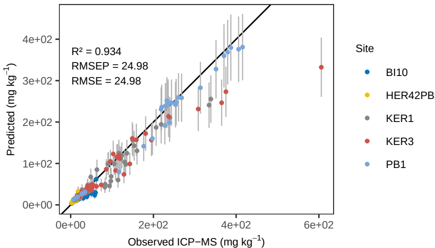
Zr RF – ACE Predicted vs Observed
