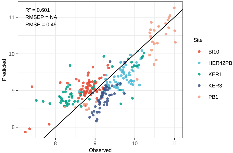
Ca OLS_weighted – Predicted vs Observed
