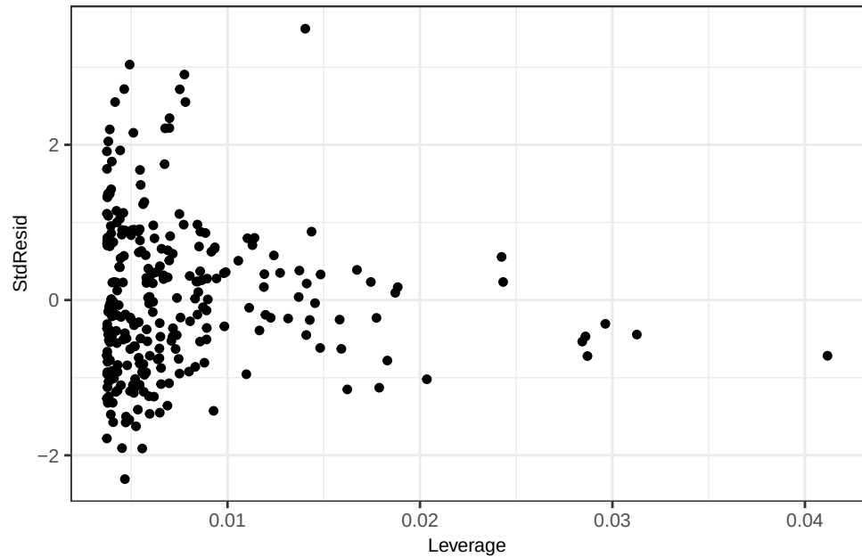
Mn OLS – Leverage
