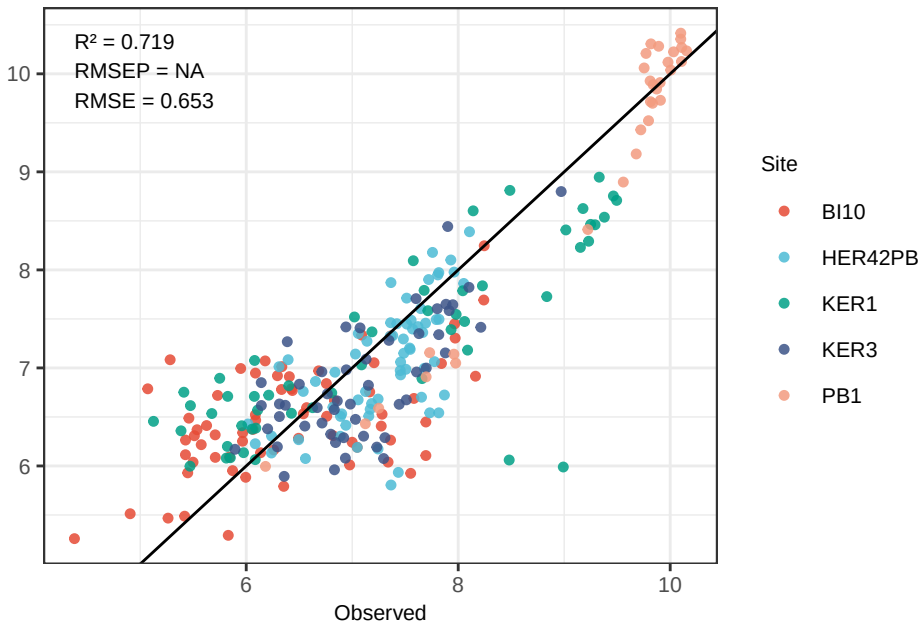
Ti OLS_weighted – Predicted vs Observed
