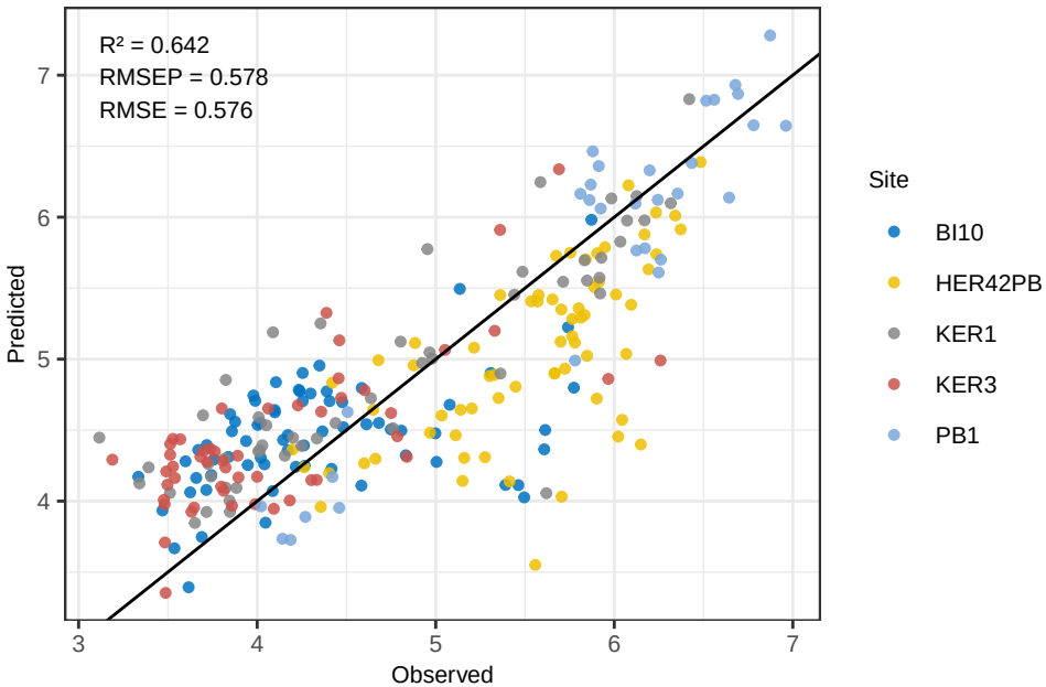
Mn OLS – Predicted vs Observed
