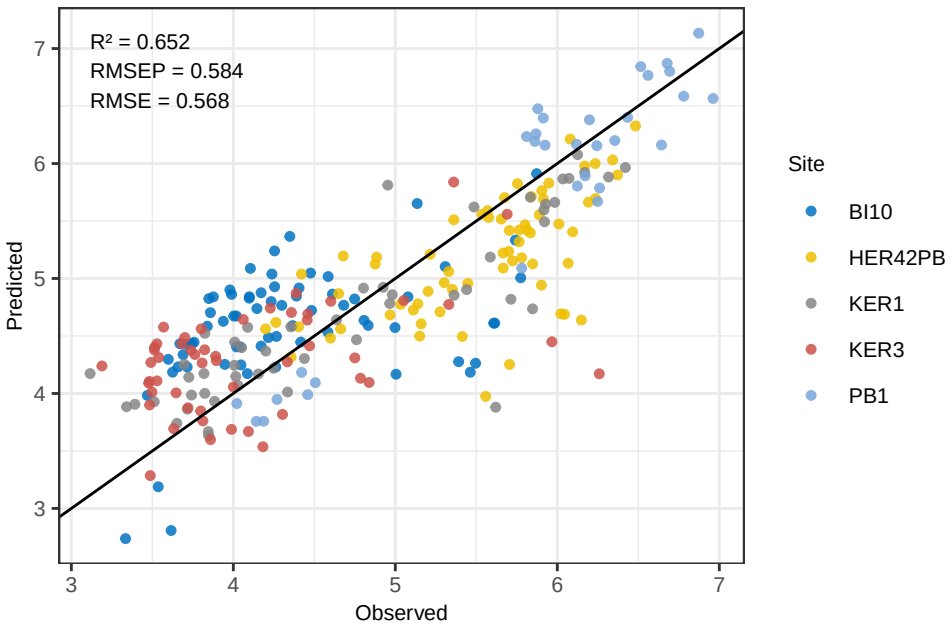
Mn PLS_LOO - Predicted vs Observed
