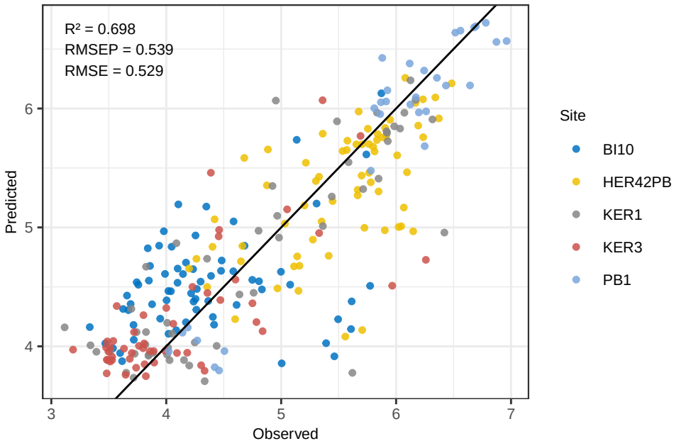
Mn RF – Predicted vs Observed
