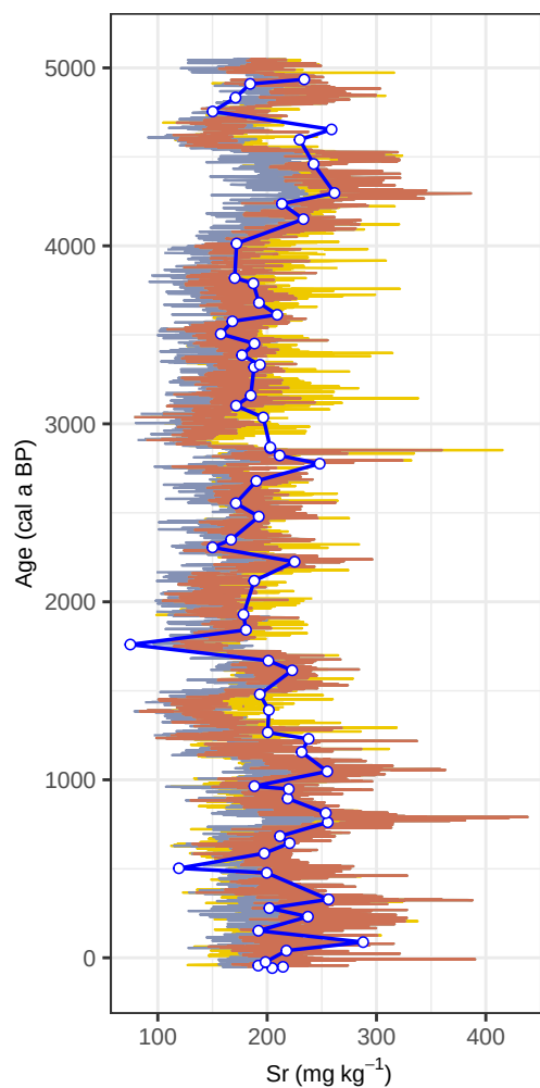
Site HER42PB – Sr (age, multivariate)
